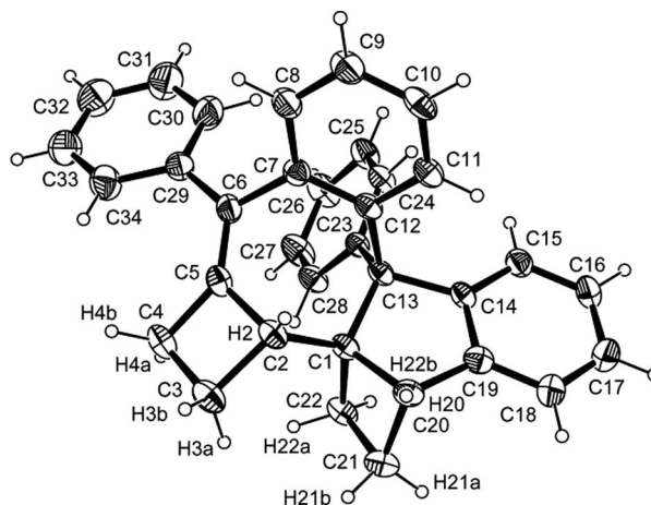
Figure 1. ORTEP-3 [12] view of the molecular structure of 11 with the atom numbering scheme. Displacement ellipsoids are drawn at 30% probability level. The hydrogen atoms are presented as small circles of arbitrary radius.
