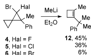
Scheme 5. Reaction of 2-methyl-2-phenyl-substituted gem -dihalogenospiropentanes with methyllithium. Yields of 12 refer to isolated product.
