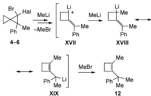
Scheme 6. Formation of product 12 .
