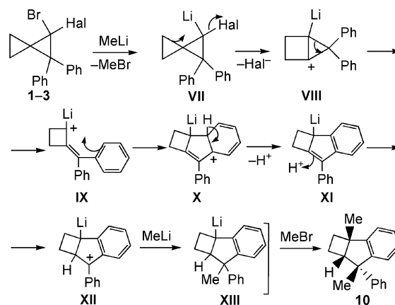
Scheme 3. Formation of tricyclic product 10 .
