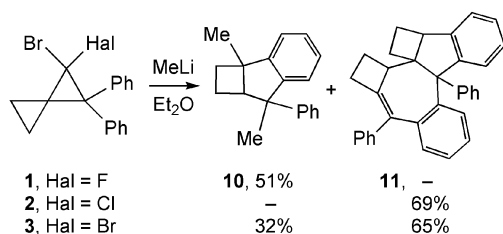
Scheme 2. Reaction of 2,2-diphenyl gem -dihalogeno-substituted spiropentanes with methyllithium.
