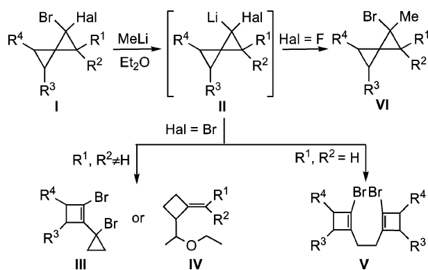
Scheme 1. Reaction of gem -dihalogenospiropentanes with methyllithium.
