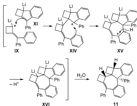
Scheme 4. Formation of fused hexocyclic system 11 .
