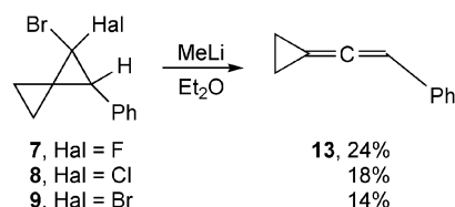
Scheme 7. Reaction of 2-phenyl-substituted gem -dihalogenospiropentanes with methyllithium.
